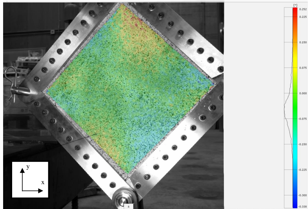
Figure 8: Specimen F2C75-02 - DIC Calculated Shear Strain
