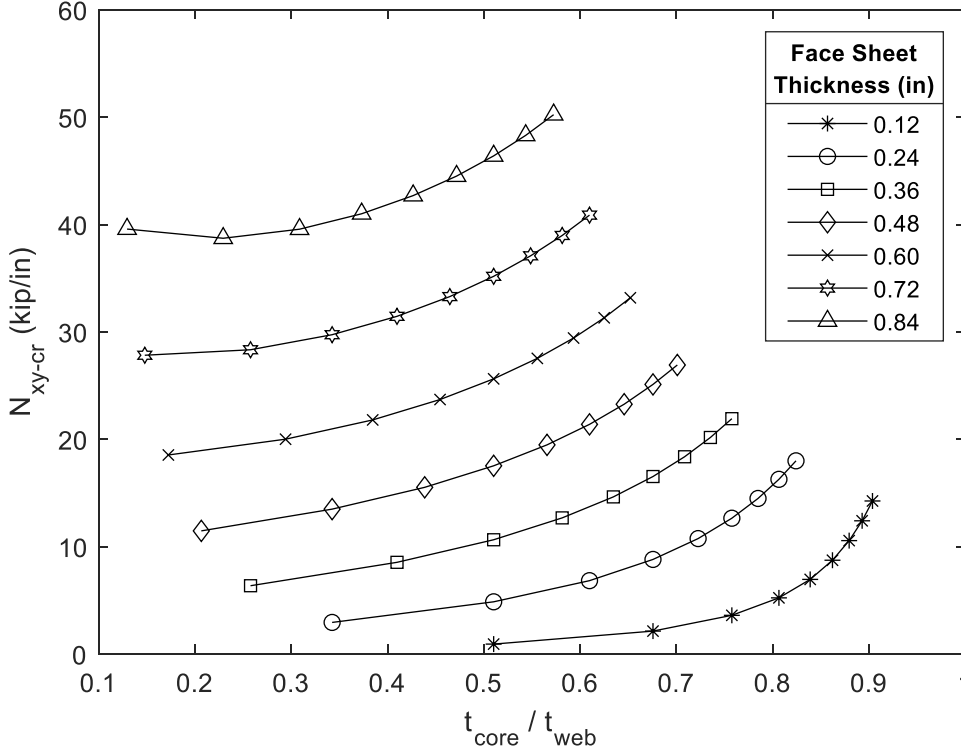
Critical Shear Buckling Stress Resultant h_{web} = 36 in
