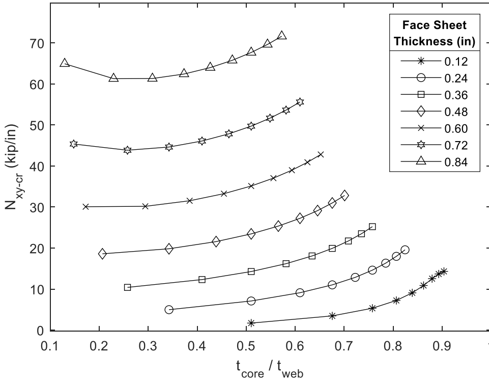
Critical Shear Buckling Stress Resultant h_{web} = 24 in
