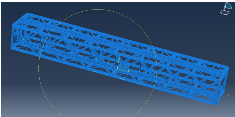
Figure 5: Track 2 and 4 of Span 3 of Cos Cob Bridge
